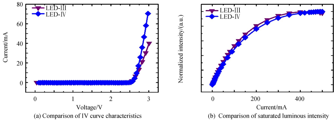
图6 LED-Ⅲ和LED-Ⅳ的性能对比 Fig. 6 Performance comparison of LED-Ⅲ and LED-Ⅳ
