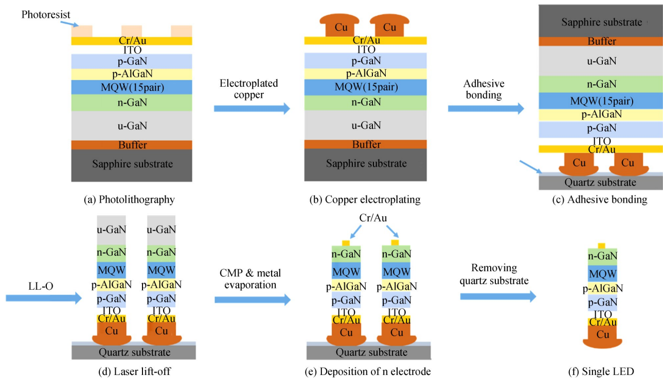
图1 GaN基自分裂垂直结构LED的工艺流程 Fig.1 Process flow of GaN-based auto-split vertical structure LED
