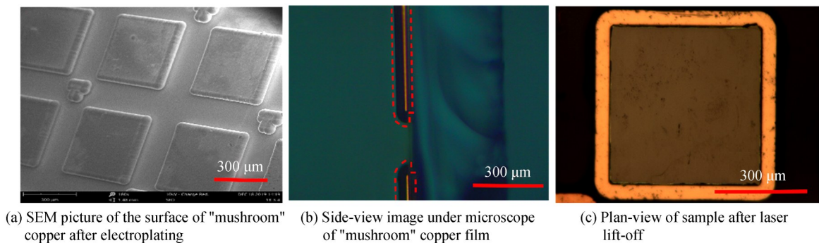
图2 蘑菇状铜衬底形貌 Fig.2 Morphology of mushroom copper substrate
